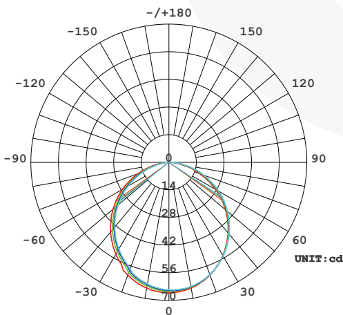
AVERAGE BEAM ANGLE (50%) : 108.4 DEG
